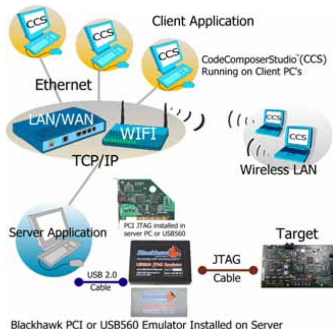
Blackhawk PCI or USB560 Emulator Installed on Server
